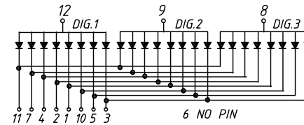
Common Anode L-KLS9-D-8031 Bx
