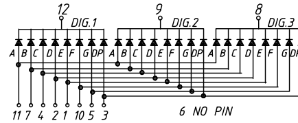
Common Cathode L-KLS9-D-8031 Ax
